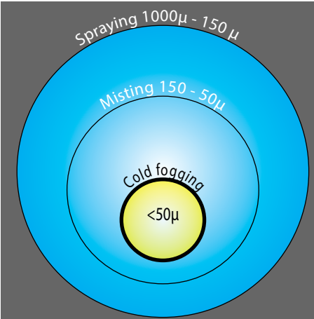
SOLO eFog 480 output data with water 20°C
