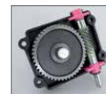
Enclosed worm drive with helical metal gears
